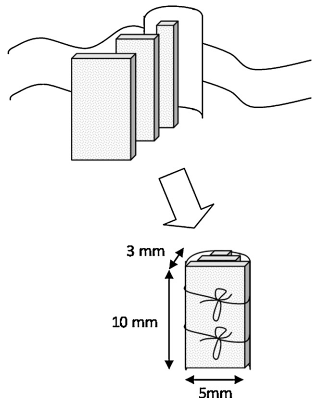
Fig. 3. Composite scaffold design.
