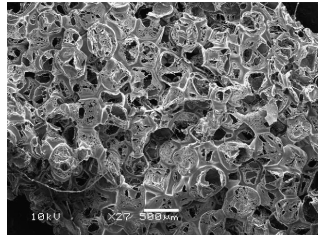
Fig. 2. Scanning electron microscope image of scaffold architecture.
