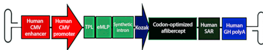
Figure 1. Design of the Aflibercept Expression Cassette (C11)
